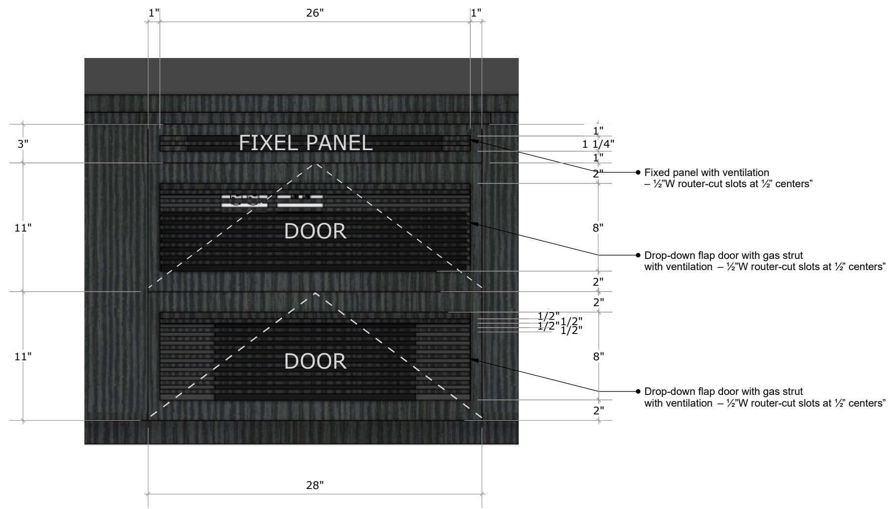
P7 DOOR DETAIL Scale: 1 1/2"=1'-0"
